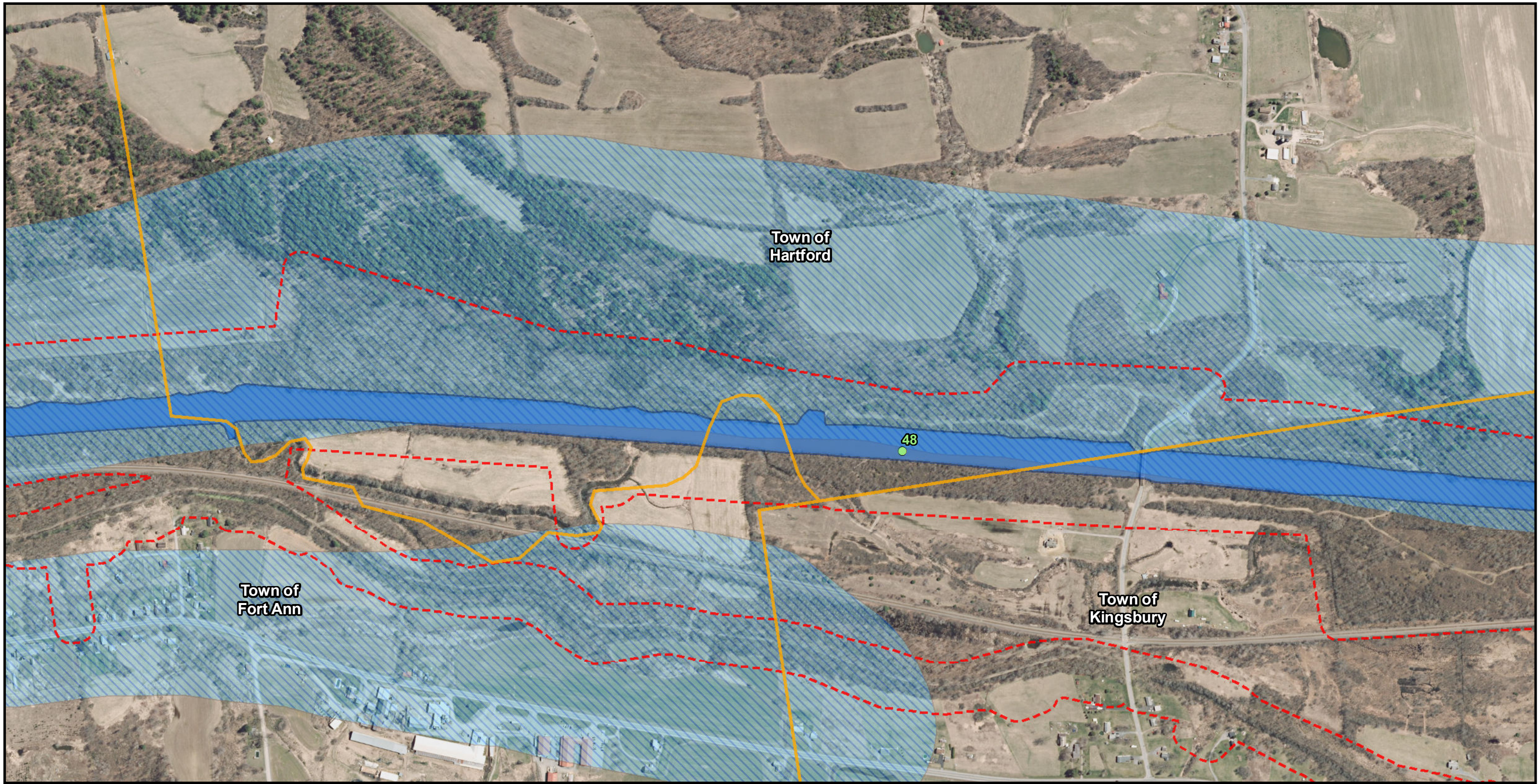
Figure 3F: Aquifers
